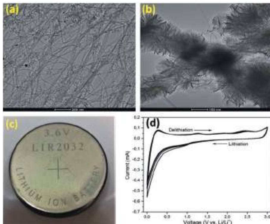
Figure 3. TEM images of (a) CNT and (b) TiO 2 nanosheet-CNT hybrid electrodes (c) photograph and (d) electrochemical performance of Li-ion battery containing CNT electrode.
